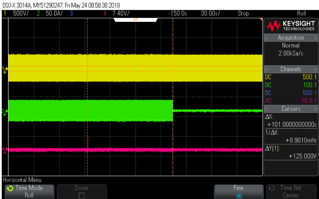
Trip time (100s setting)
